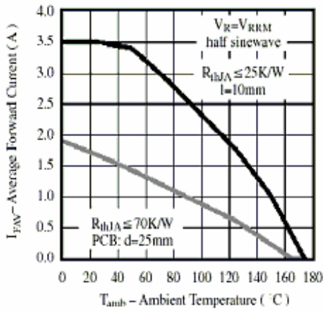
Figure 3. Max. Average Forward Current vs. Ambient Temperature
