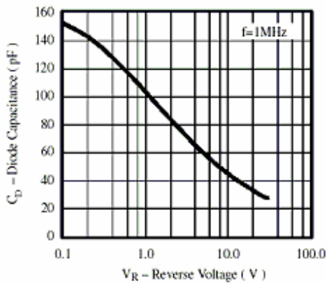
Figure 5. Typ. Diode Capacitance vs. Reverse Voltage
