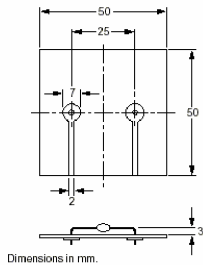
Figure 6. Device mounted on a printed-circuit board.
