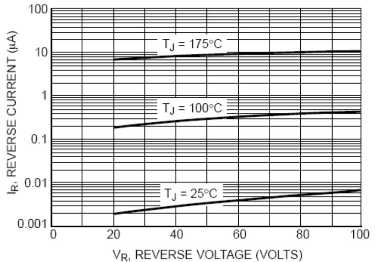
Fig.4- Typical Reverse Current
