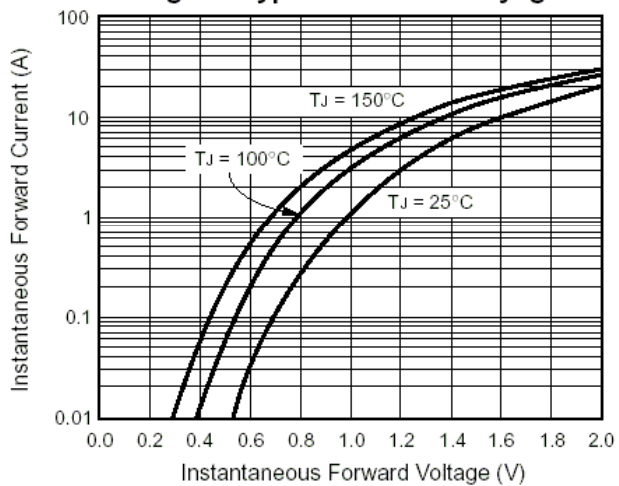
Fig. 4 – Typical Forward Volyage
