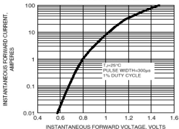
FIG. 5 - TYPICAL INSTANTANEOUS FORWARD CHARACTERISTICS PER LEG
