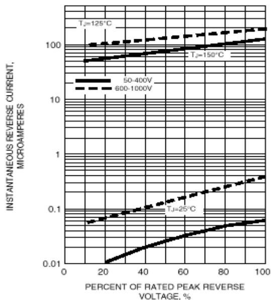
FIG. 6 - TYPICAL REVERSE LEAKAGE CHARACTERISTICS PER LEG
