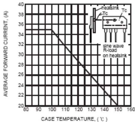
Figure 7. Typical Forward Current Derating Curve
