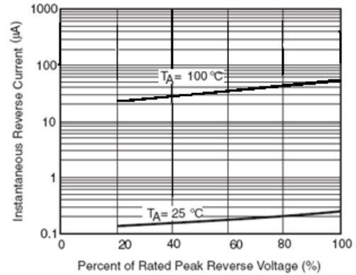
Figure 4. Typical Reverse Characteristics Per Leg
