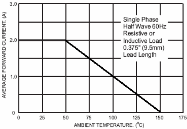
FIG.1- MAXIMUM AVERAGE FORWARD CURRENT DERATING
