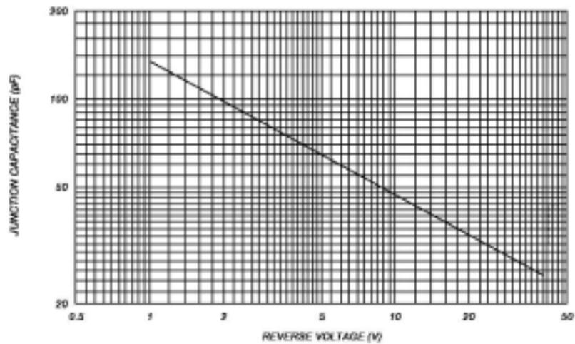
JUNCTION CAPACITANCE VS. REVERSE VOLTAGE
