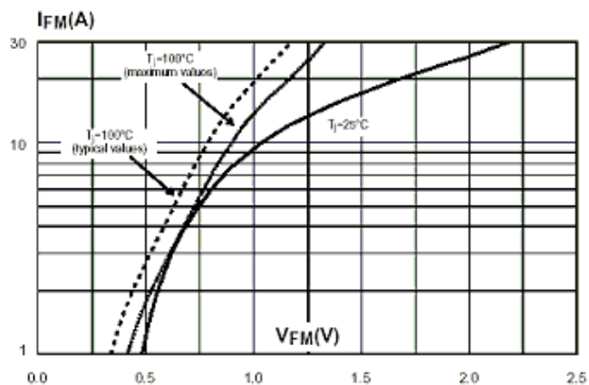
Fig.4 : Forward voltage drop versus forward current (high level, maximum values).
