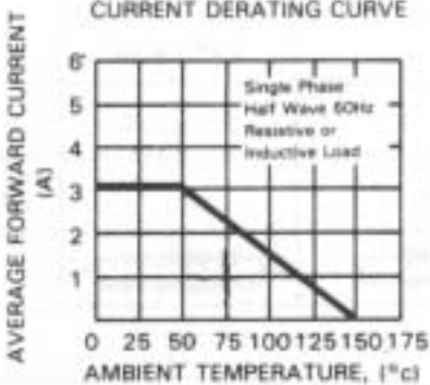
FIG. 5 - TYPICAL FORWARD CURRENT DERATING CURVE
