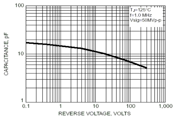
FIG. 6 - TYPICAL JUNCTION CAPACITANCE PER LEG
