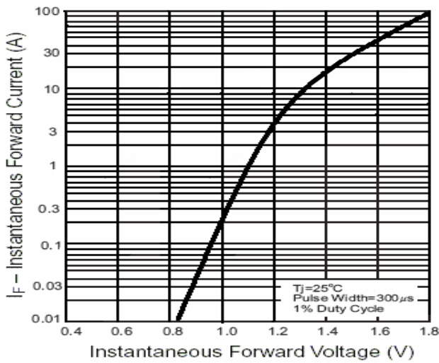
Typical Instantaneous Forward Characteristics Per Leg
