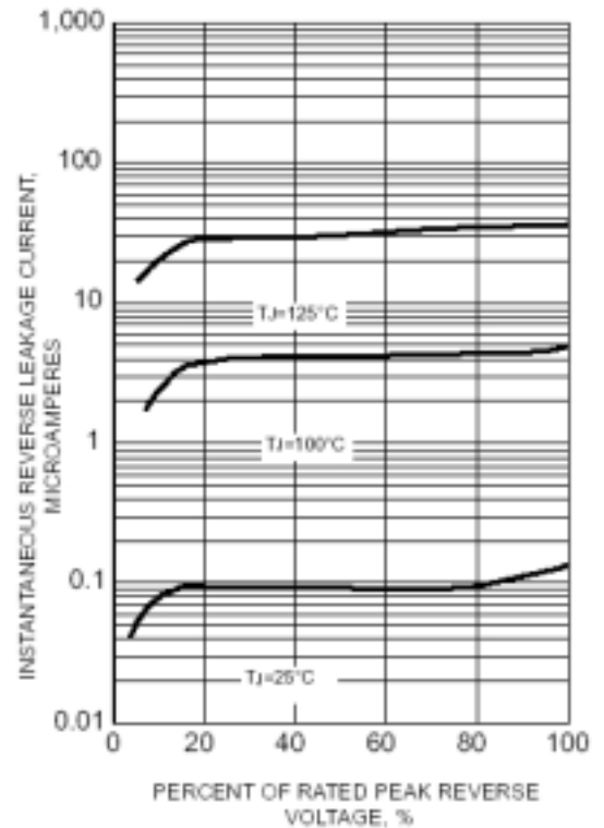
FIG. 4 - TYPICAL REVERSE LEAKAGE CHARACTERISTICS
